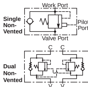
MHC-010-S*S* Non-Vented Counterbalance Adjustable
