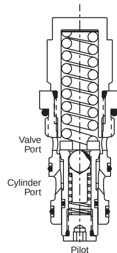
MHC-022-S*N* Non-Vented Counterbalance Non-Adjustable
